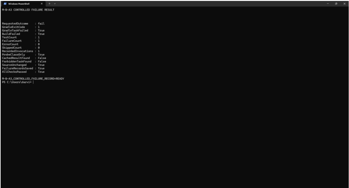
Figure 2. One test failed as requested. Gradle returned exit code 1 and marked the task as failed.
